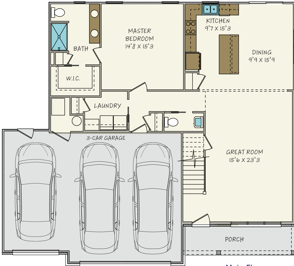
Main Floor
